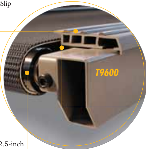
One-inch Prewaxed Phenolic Deck
